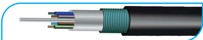
48,96 CORE SINGLE MODE INDOOR/OUTDOOR ARMoured FIBER OPTIC CABLE G.652D
